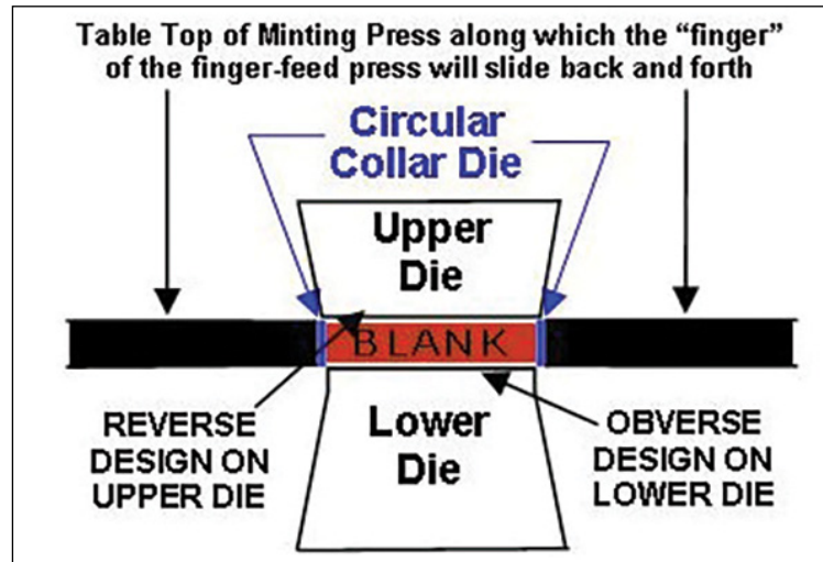
Figure 2. A side view of the finger feed press shows the position of the dies at the moment a blank is struck.
